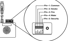
Figure 3: Conexiones de Contact Closure [Cierre de Contacto] EnviroSense
